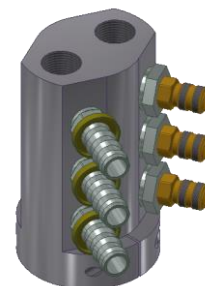
Air distributor
