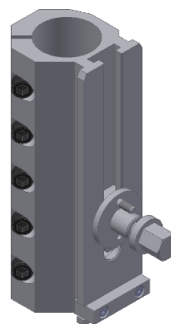
Mounting Kit for Emhart Blow Head Holder 5": 215F126100
